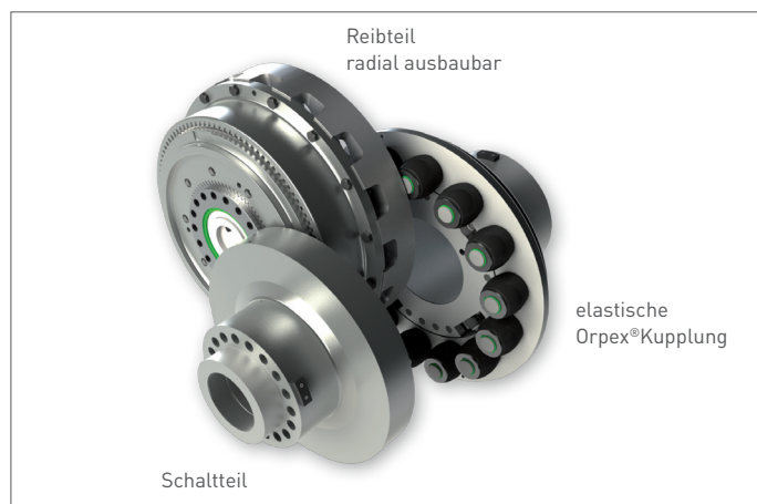
Bauart PPF-RA-Orpex®
